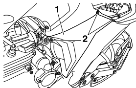
1. Painel A 2. Parafuso
